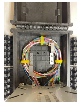
Fiber cable storage
